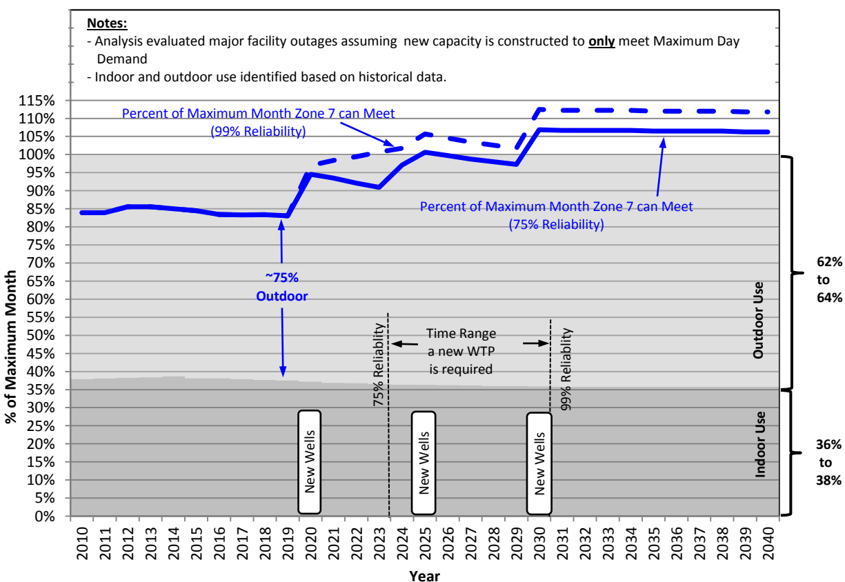
Figure 10-21. Ability of In-Valley Portfolio to Meet Maximum Month Demand during an Outage
