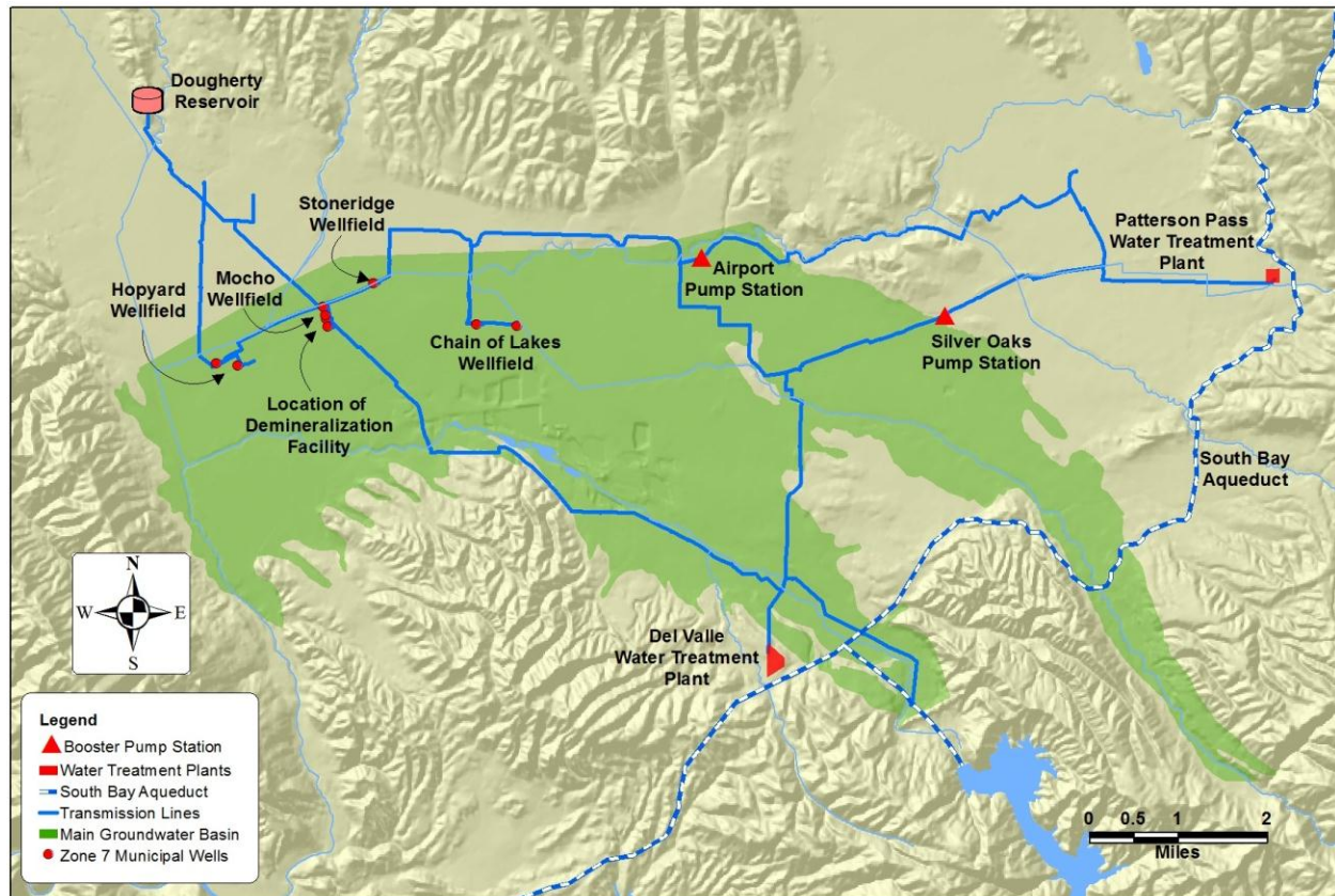
Figure 4-5. Zone 7's Major Treated Water System Facilities
