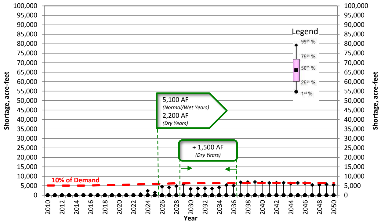
Figure 11-11. Reliability Curve for the Intertie Portfolio: 90%
