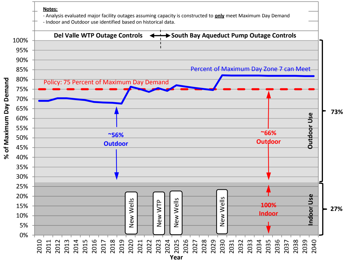
Figure 11-20. Ability of the Intertie Portfolio to Meet Maximum Day Demand during an Outage
