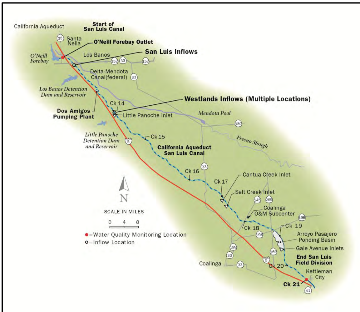
Figure 14-19. Location of Non-Project Inflows in the San Luis Canal Reach of the California Aqueduct
