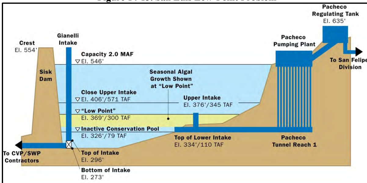
Figure 14-13. San Luis Low-Point Problem
