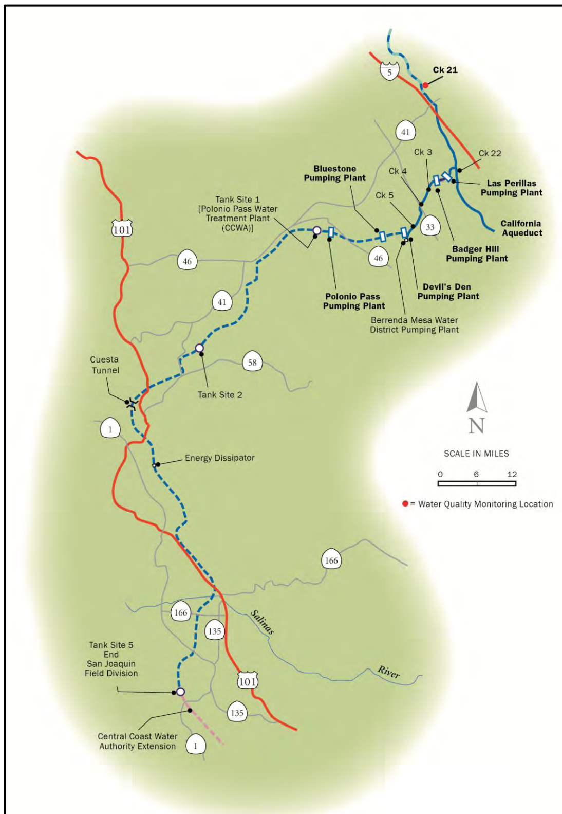
Figure 14-15. Coastal Branch Facilities
