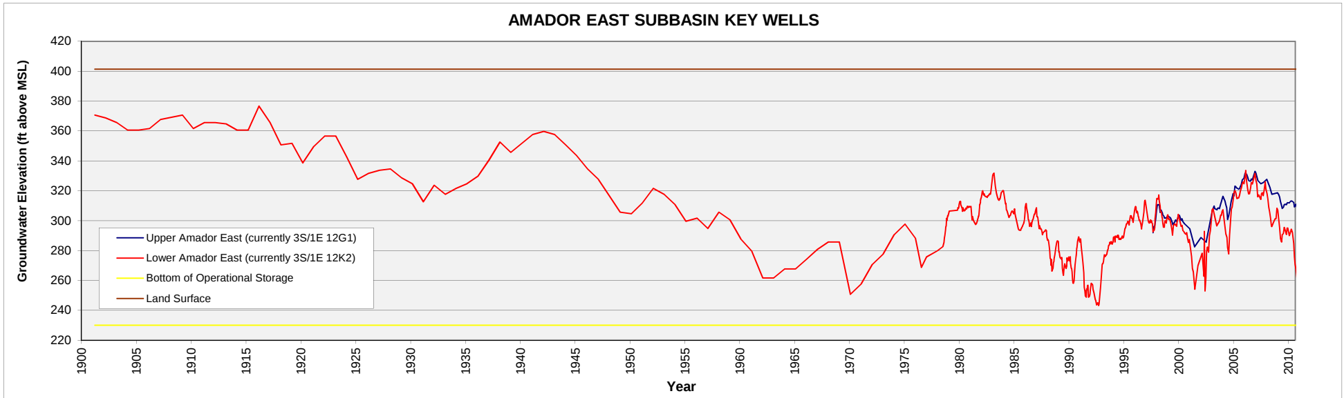
FIGURE 3.2-2 ZONE 7 WATER AGENCY Key Well Hydrographs - Historical Eastern Portion of Main Basin
