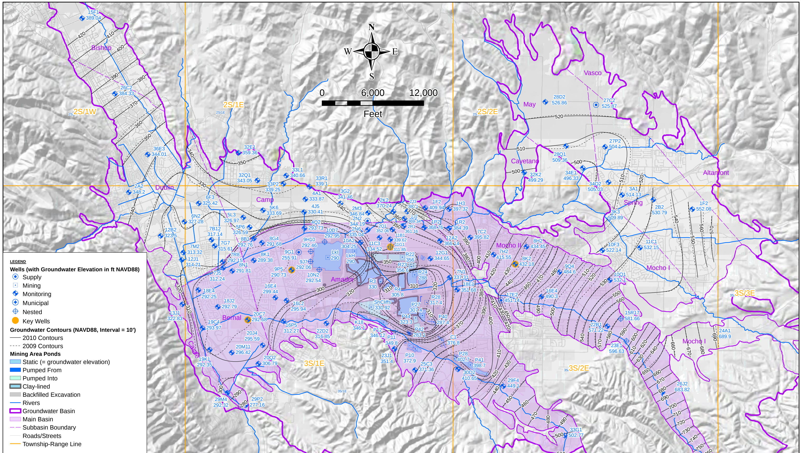
Figure 3.2-4 Groundwater Gradient Map Upper Aquifer; Spring 2010 (April) Livermore Valley Groundwater Basin
