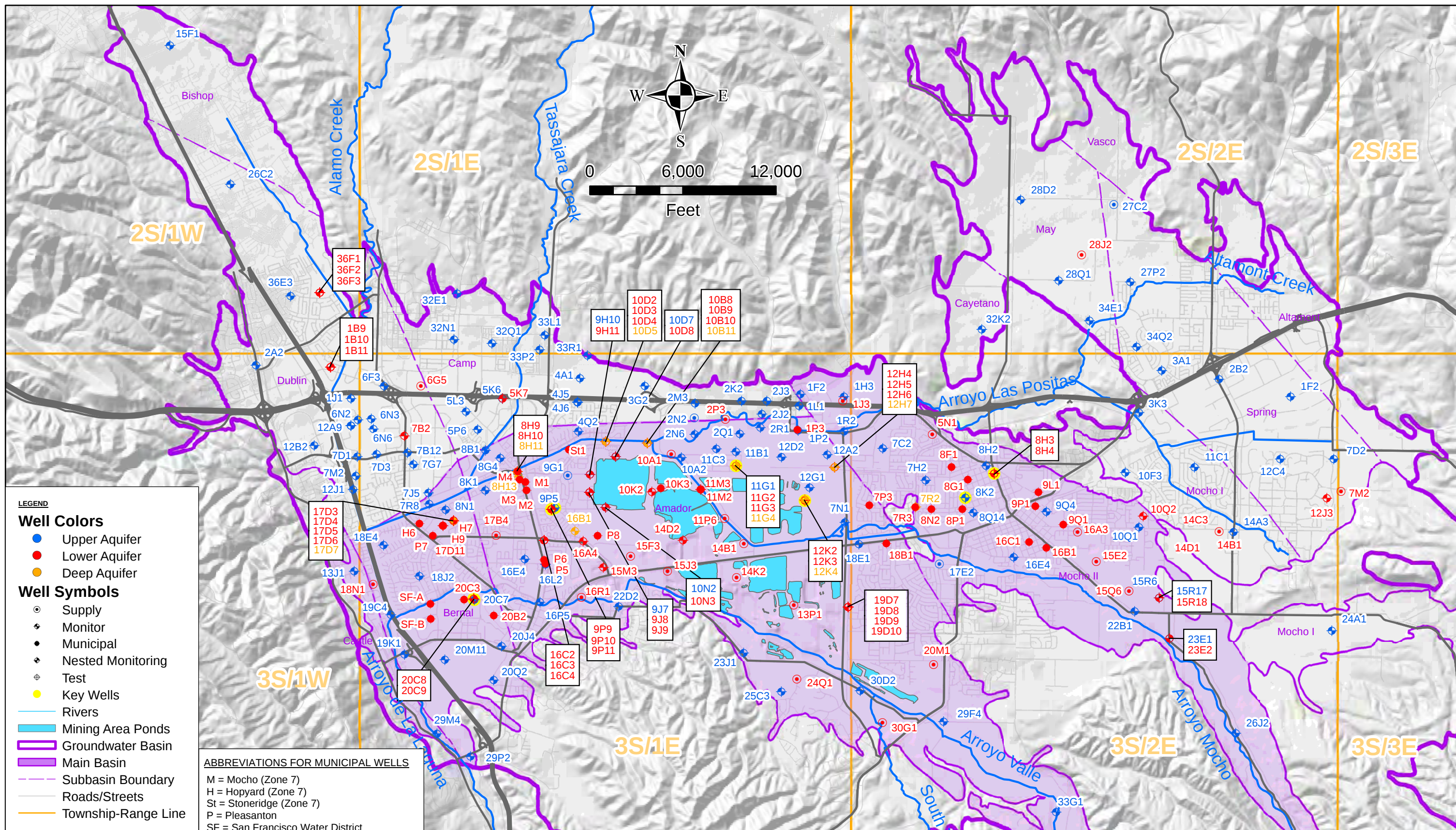
Figure 3.2-1 Zone 7 Groundwater Program Wells in 2010 Program Livermore Valley Groundwater Basin
