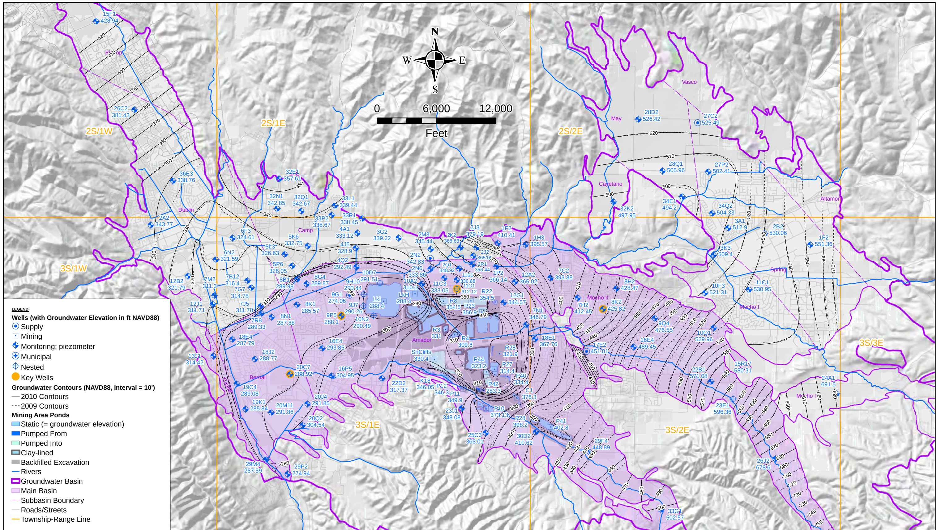
Figure 3.2-5 Groundwater Gradient Map Upper Aquifer; Fall 2010 (September) Livermore Valley Groundwater Basin
