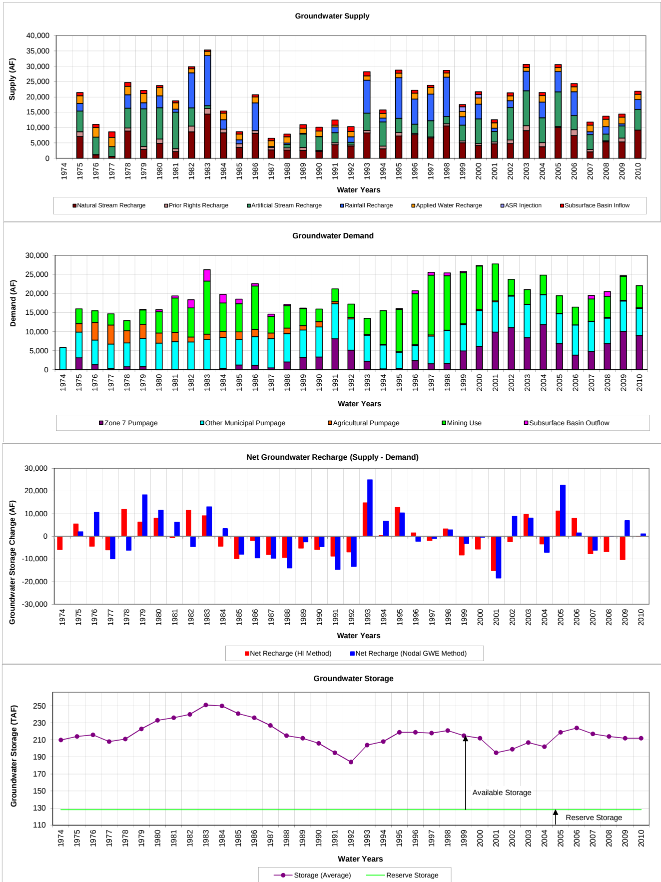
Figure 4.2-2 Graphs of Historical Main Basin Hydrologic Inventory 1974 to 2010 Water Years
