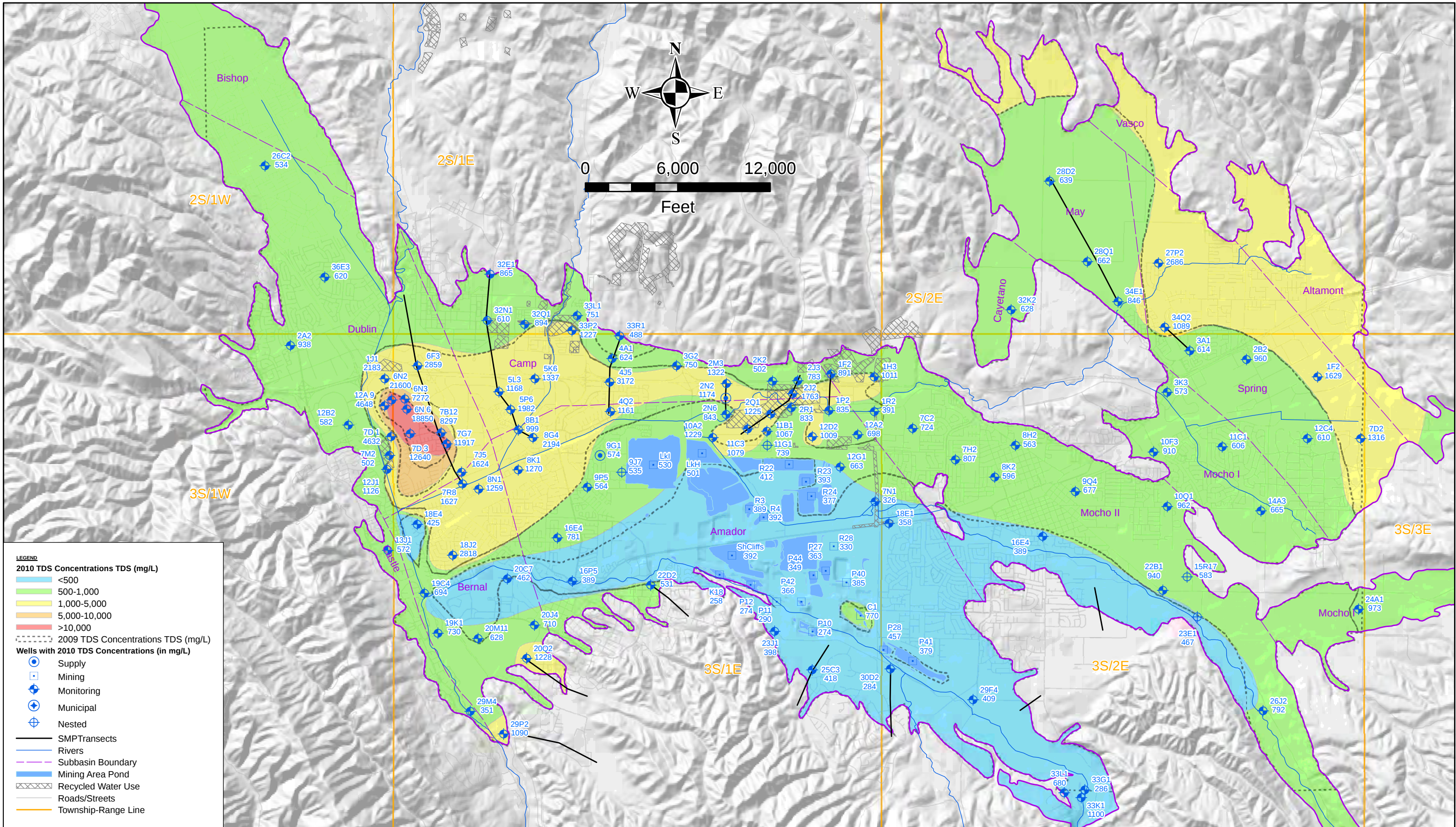
Figure 3.2-9 TDS Concentrations (mg/L) Upper Aquifer; 2010 Water Year Livermore Valley Groundwater Basin
