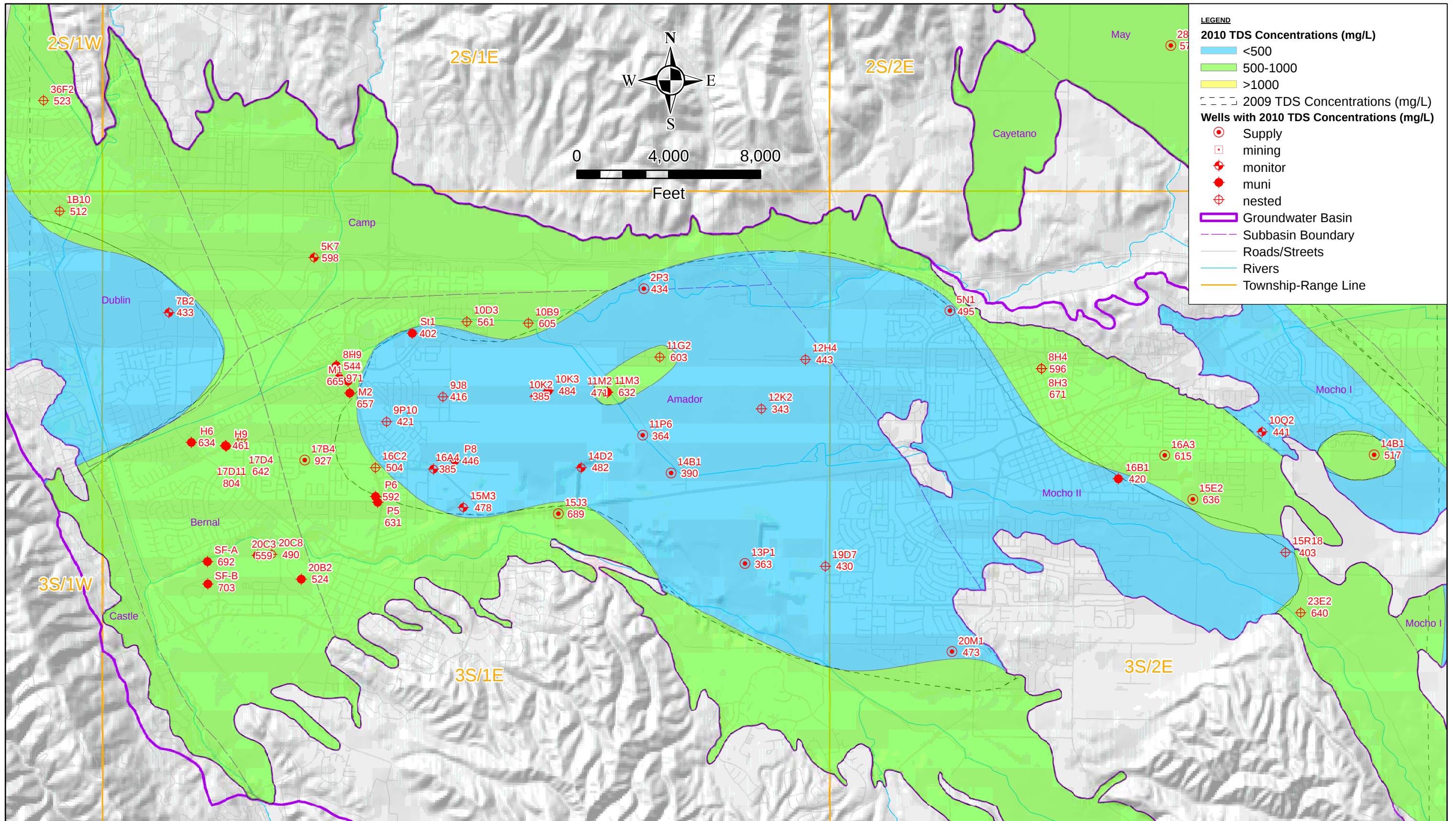
Figure 3.2-12 TDS Concentrations (mg/L) Lower Aquifer; 2010 Water Year Livermore Valley Groundwater Basin
