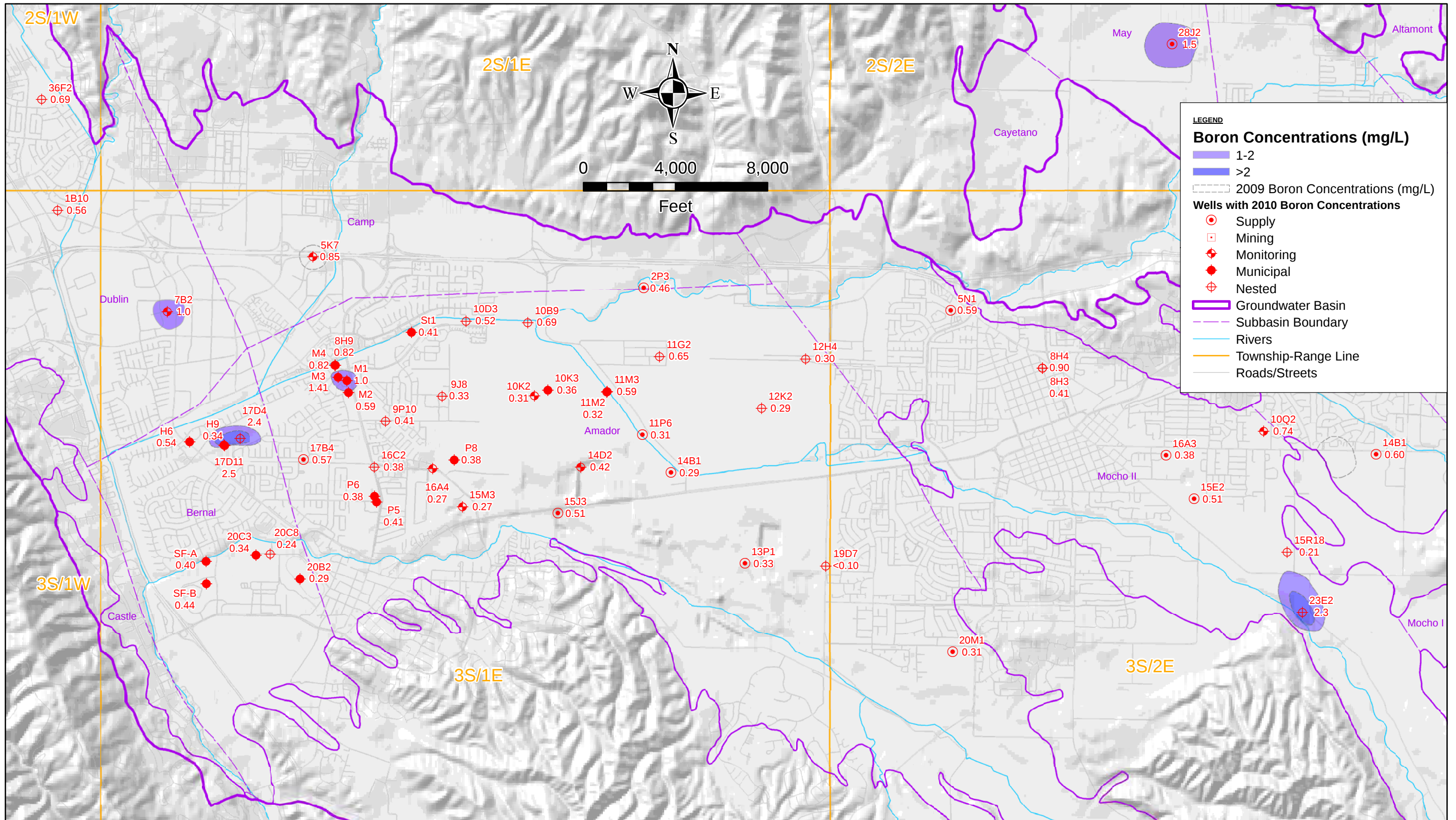
Figure 3.2-14 Boron Concentrations (mg/L) Lower Aquifer; 2010 Water Year Livermore Valley Groundwater Basin
