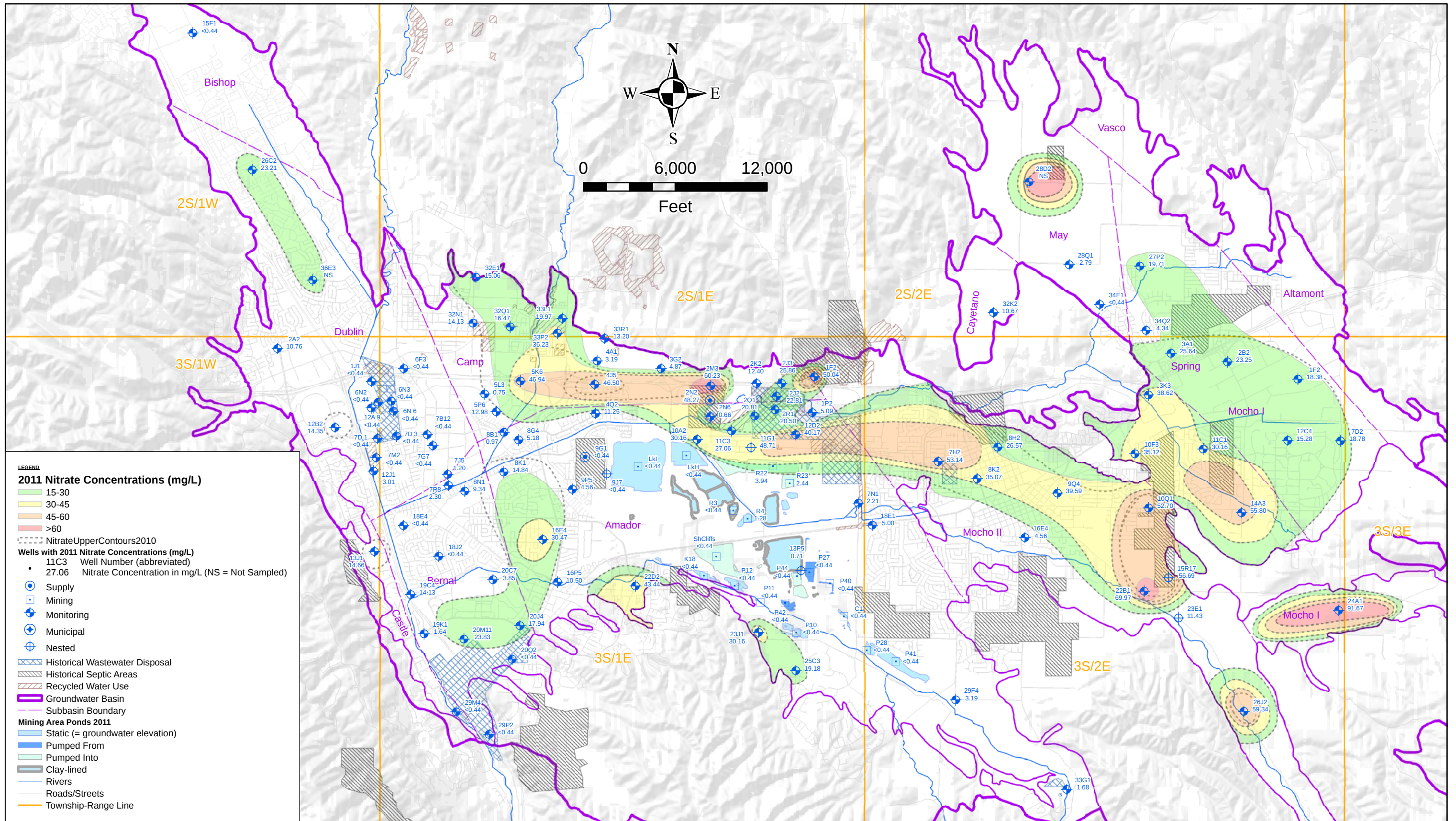
Figure 3.2-10 Nitrate Concentrations (mg/L) Upper Aquifer; 2011 Water Year Livermore Valley Groundwater Basin
