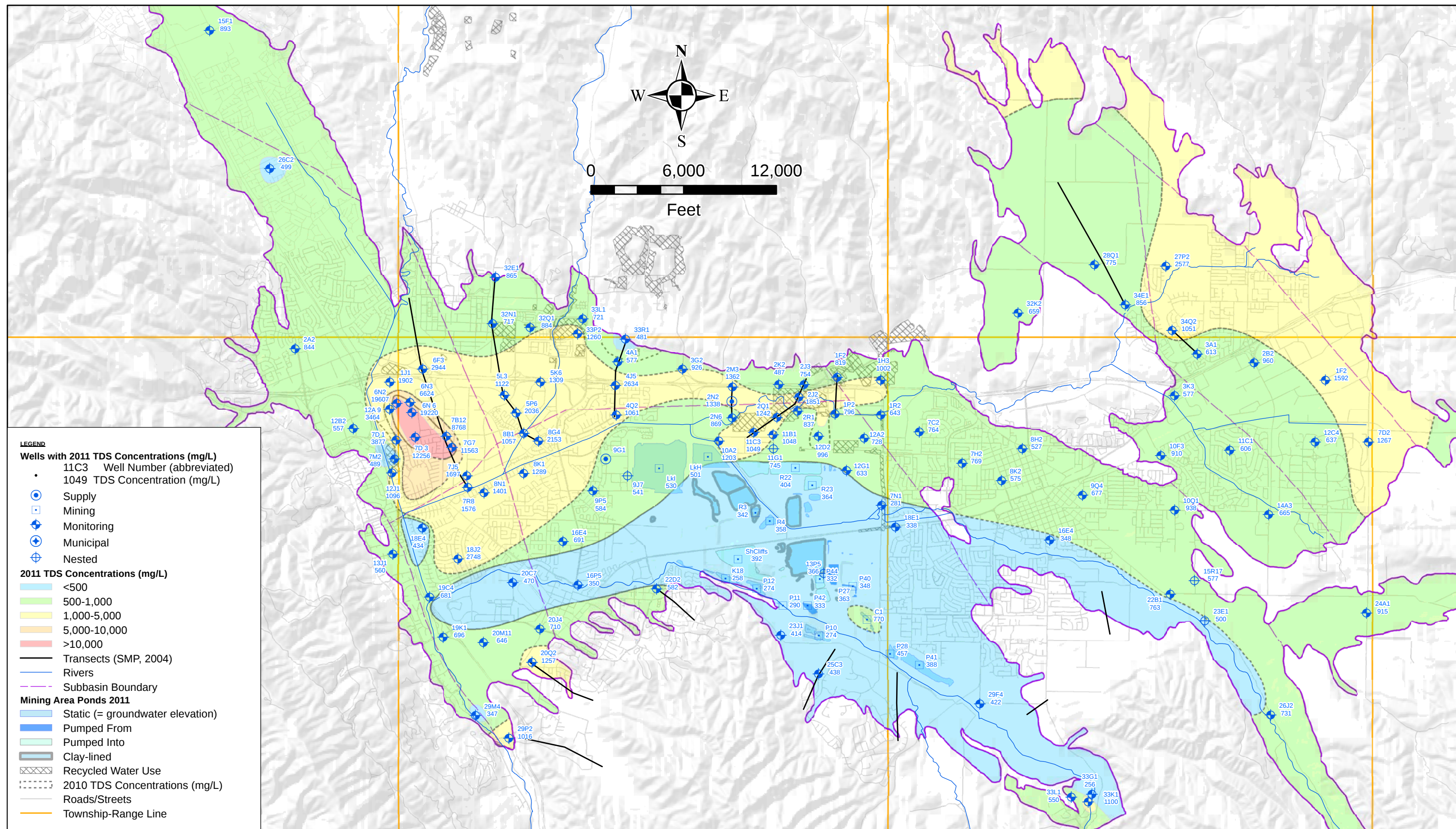
Figure 3.2-9 TDS Concentrations (mg/L) Upper Aquifer; 2011 Water Year Livermore Valley Groundwater Basin
