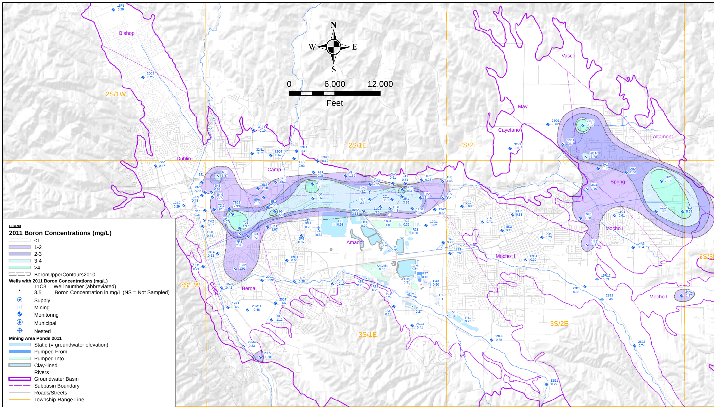
Figure 3.2-11 Boron Concentrations (mg/L) Upper Aquifer; 2011 Water Year Livermore Valley Groundwater Basin
