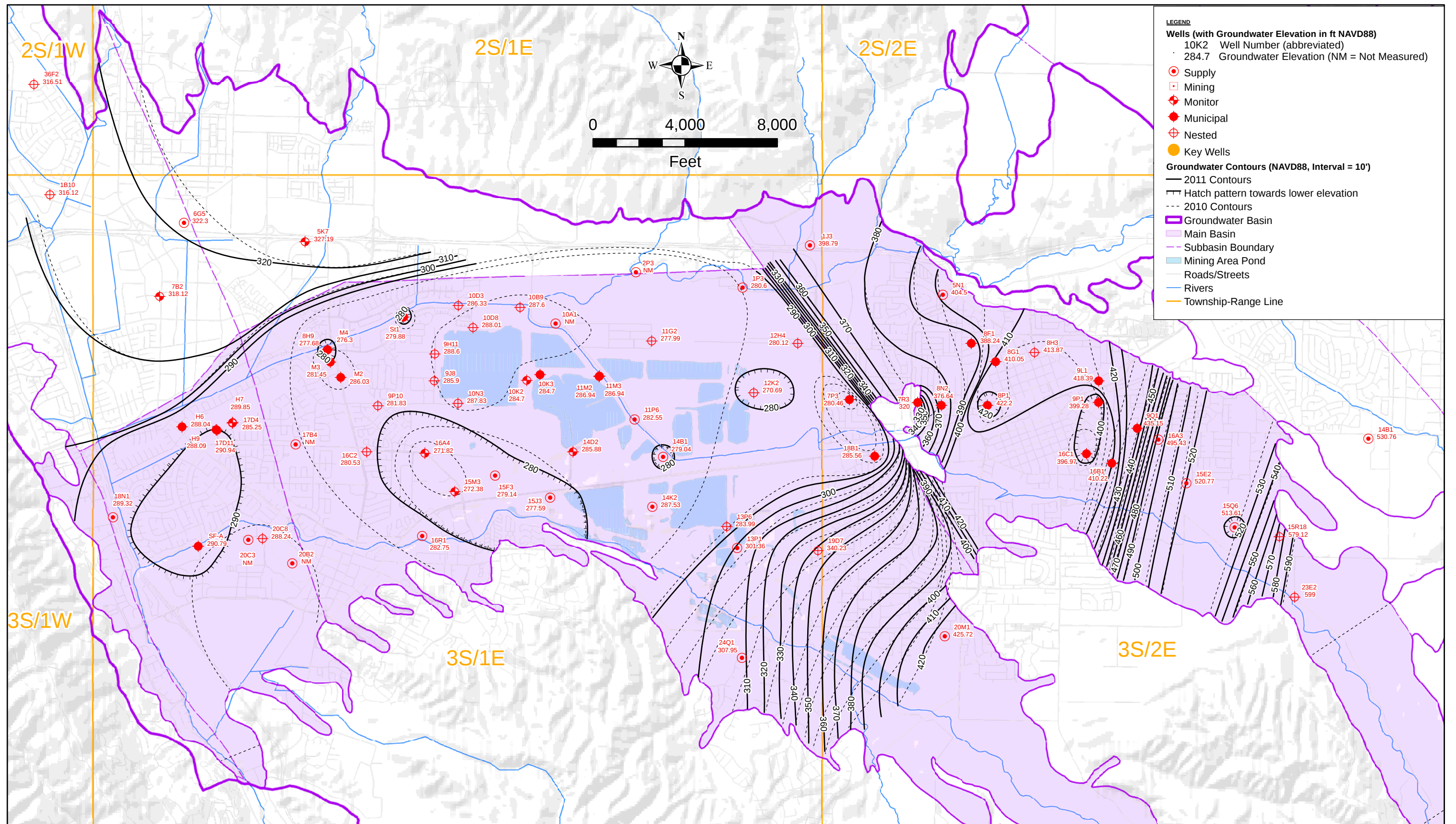
Figure 3.2-7 Groundwater Gradient Map Lower Aquifer; Fall 2011 (September) Livermore Valley Groundwater Basin
