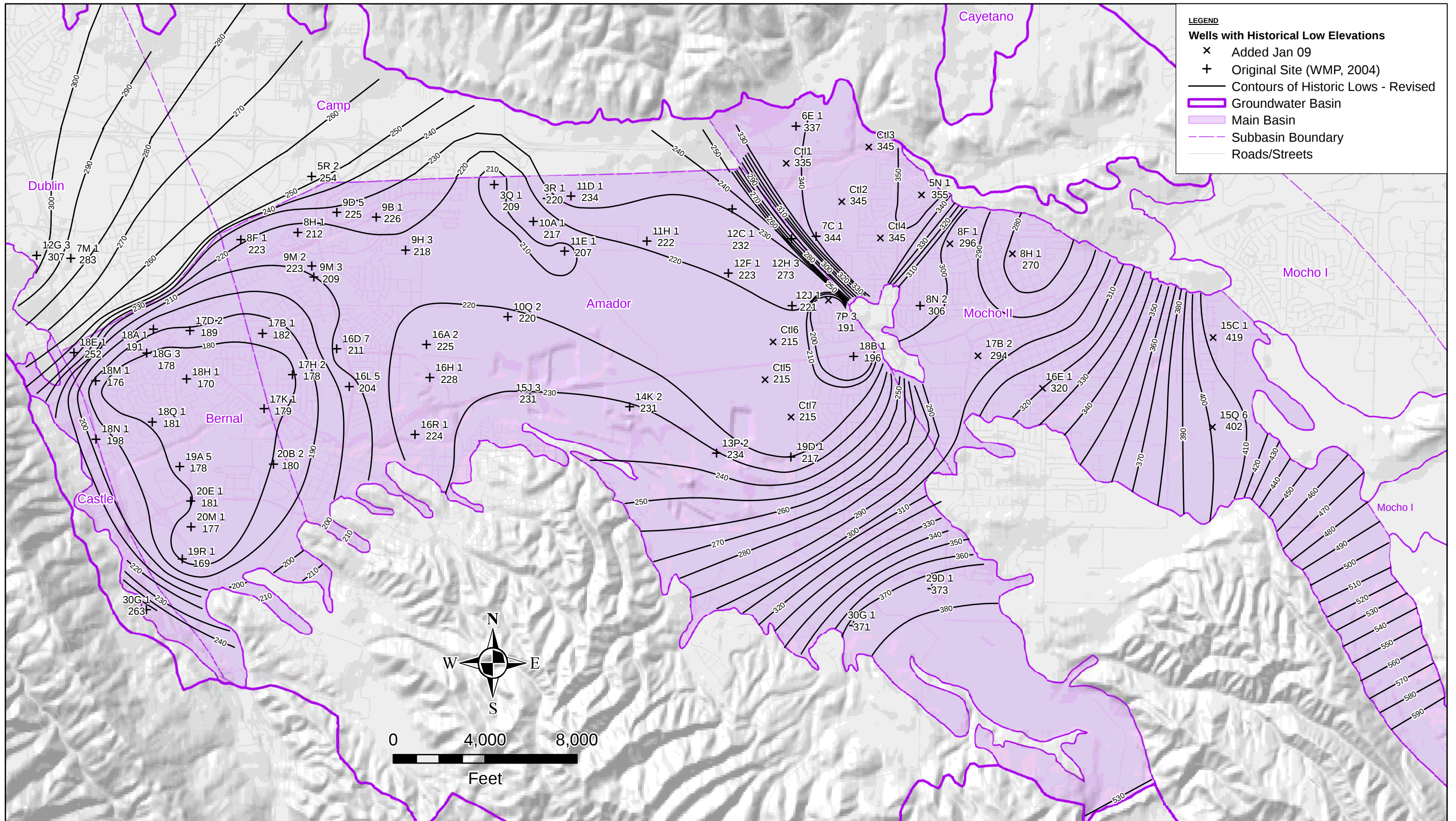
Figure 2.2-3 Historical Lows (Update Jan 2009) Lower Aquifer Livermore Valley Groundwater Basin
