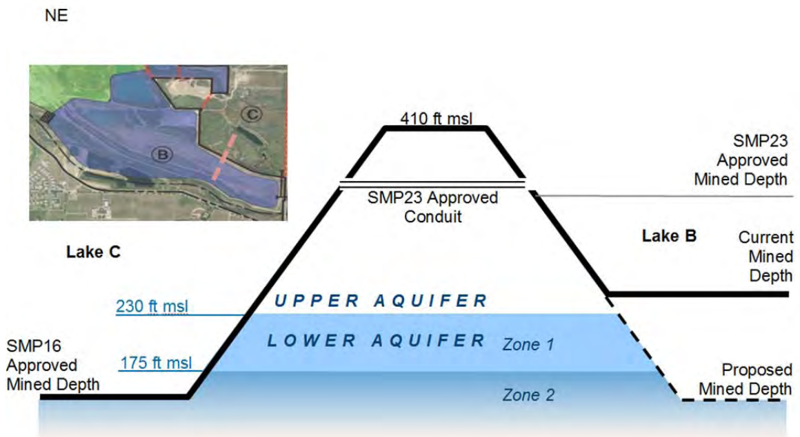
Figure 3-9. Proposed modifications to Lake B (CEMEX Reclamation Plan Amendment, June 2013).
